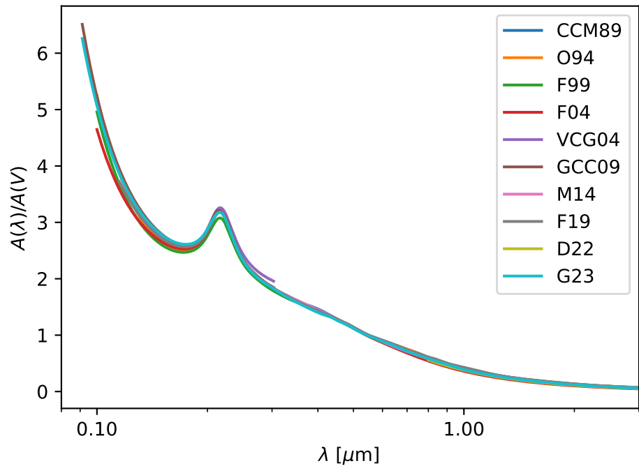
UV-NIR R(V) = 3.1
