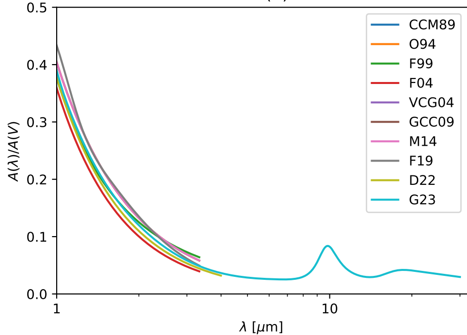
NIR-MIR R(V) = 3.1
