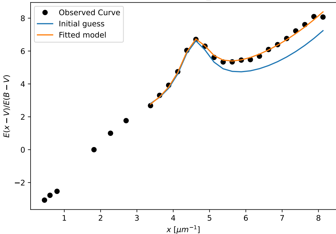
Example FM90 Fit to G03_LMCAvg curve
