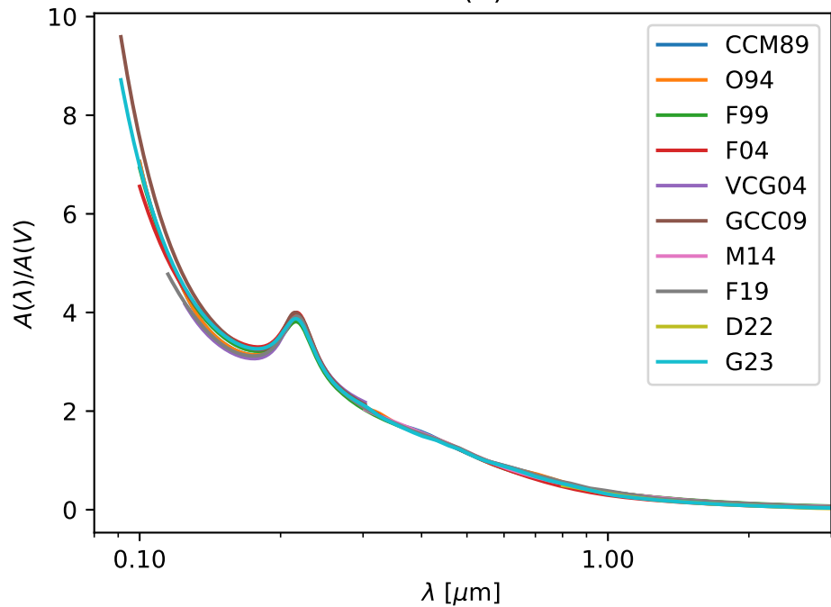
UV-NIR R(V) = 2.5
