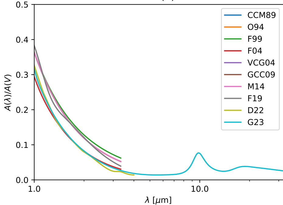
NIR-MIR R(V) = 2.5
