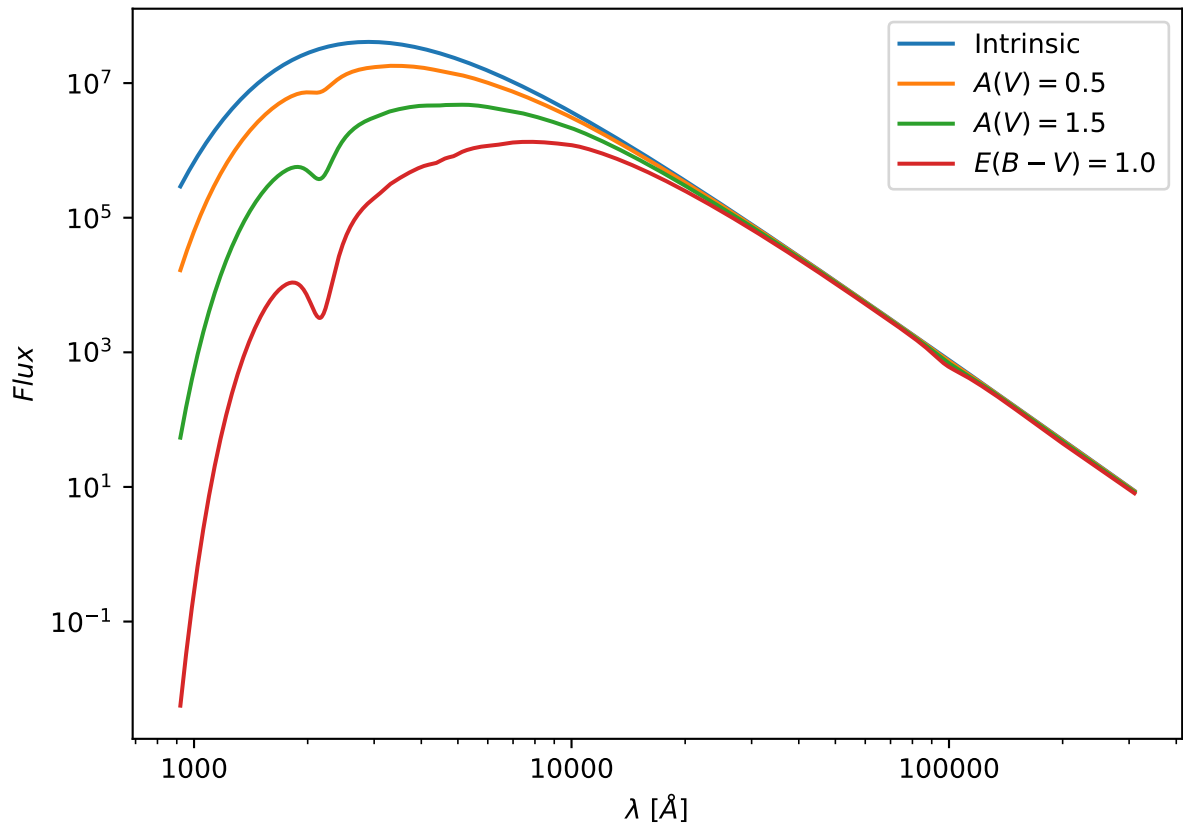
Example extinguishing a blackbody
